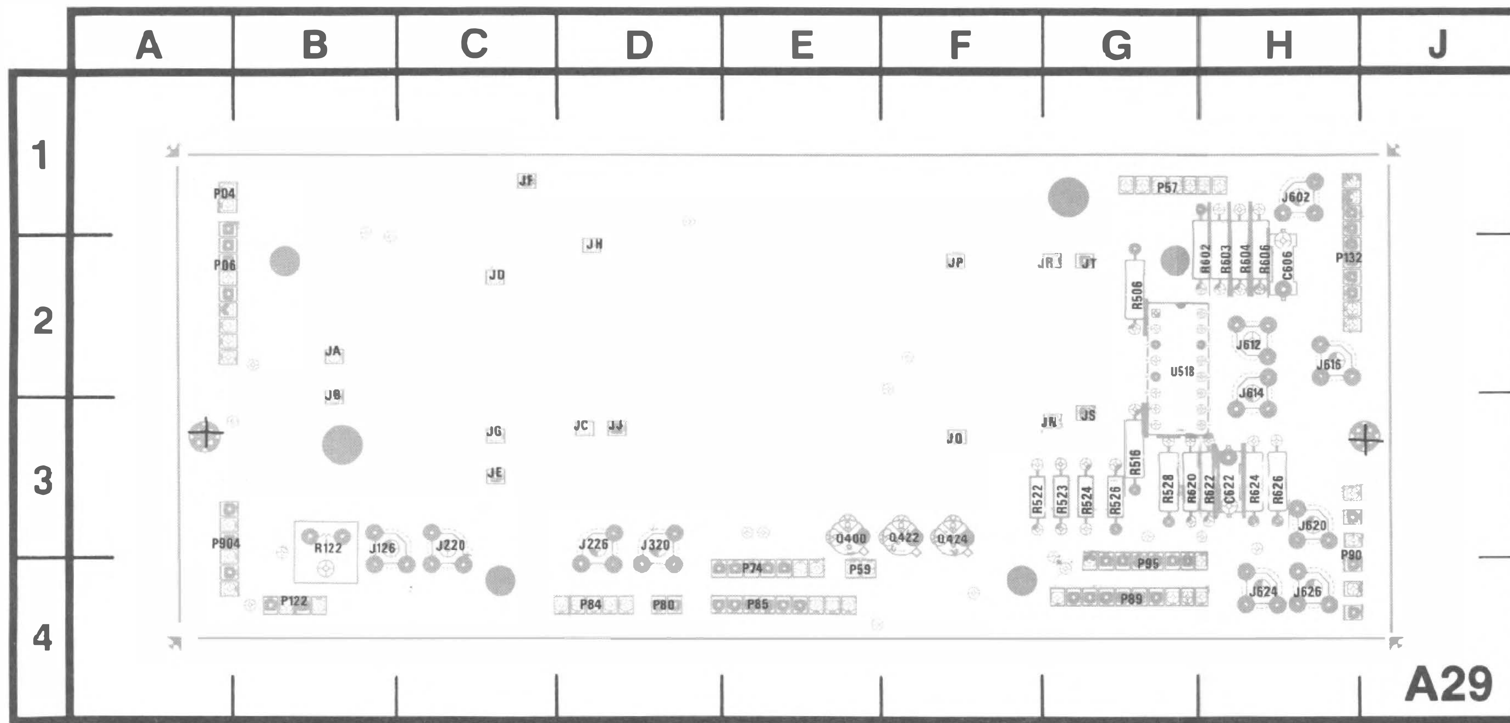
Figure 8-13. A29—Horizontal Interface circuit board assembly.
