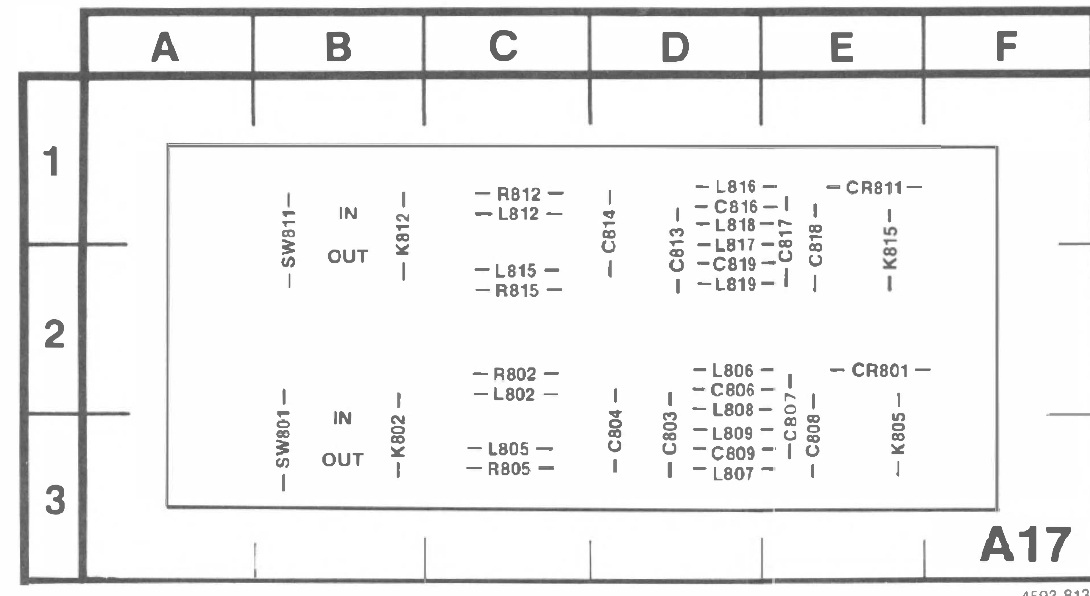
Figure 8-14. A17—X-Y Delay Compensation (Option 2) circuit board assembly.
