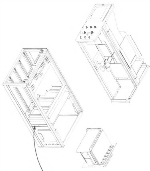
Figure 8-6. A13—Logic circuit board assembly.
