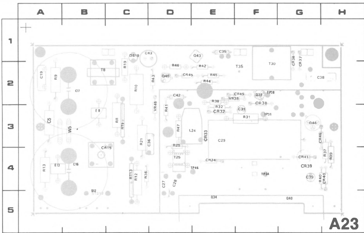
Figure 8-18. A23—Inverter circuit board assembly.
