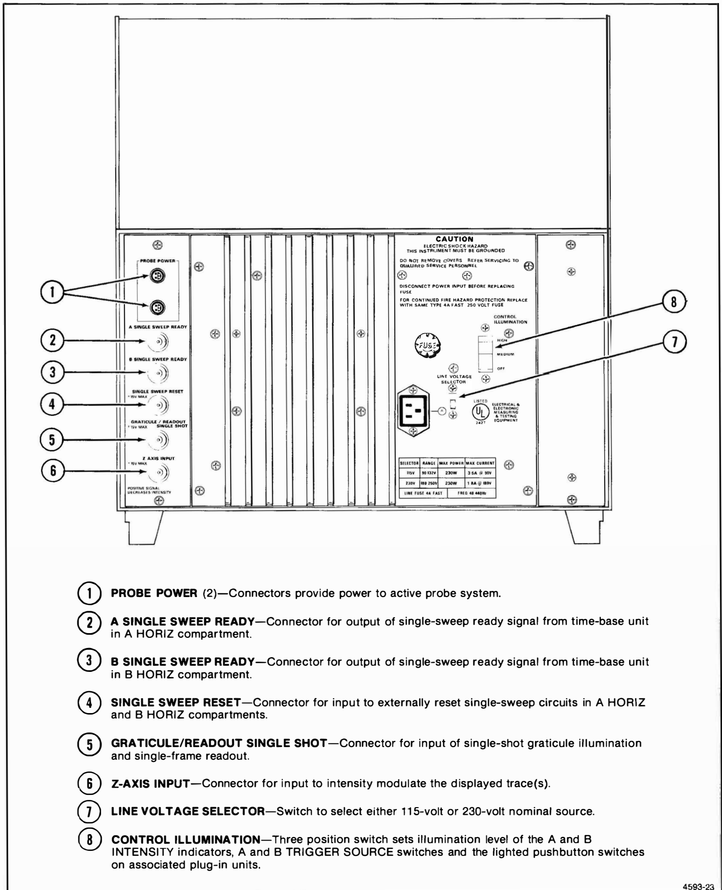
Figure 2-2. Rear-panel controls and connectors.
