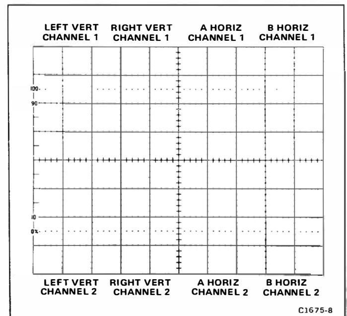
Figure 2-4. Location of readout on the crt identifying the originating plug-in and channel.
