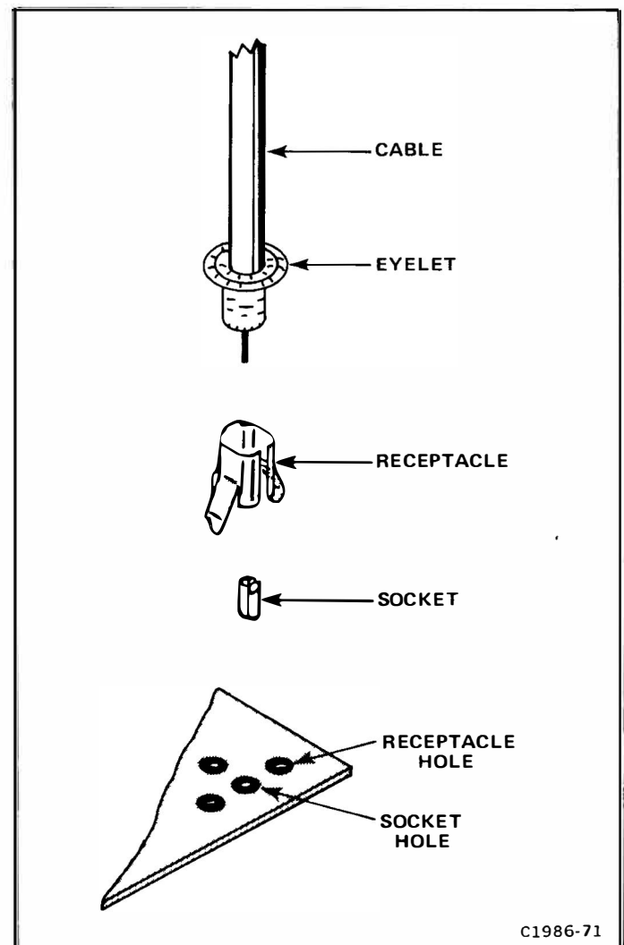
Figure 4-15. Coaxial end-lead connector assembly.
