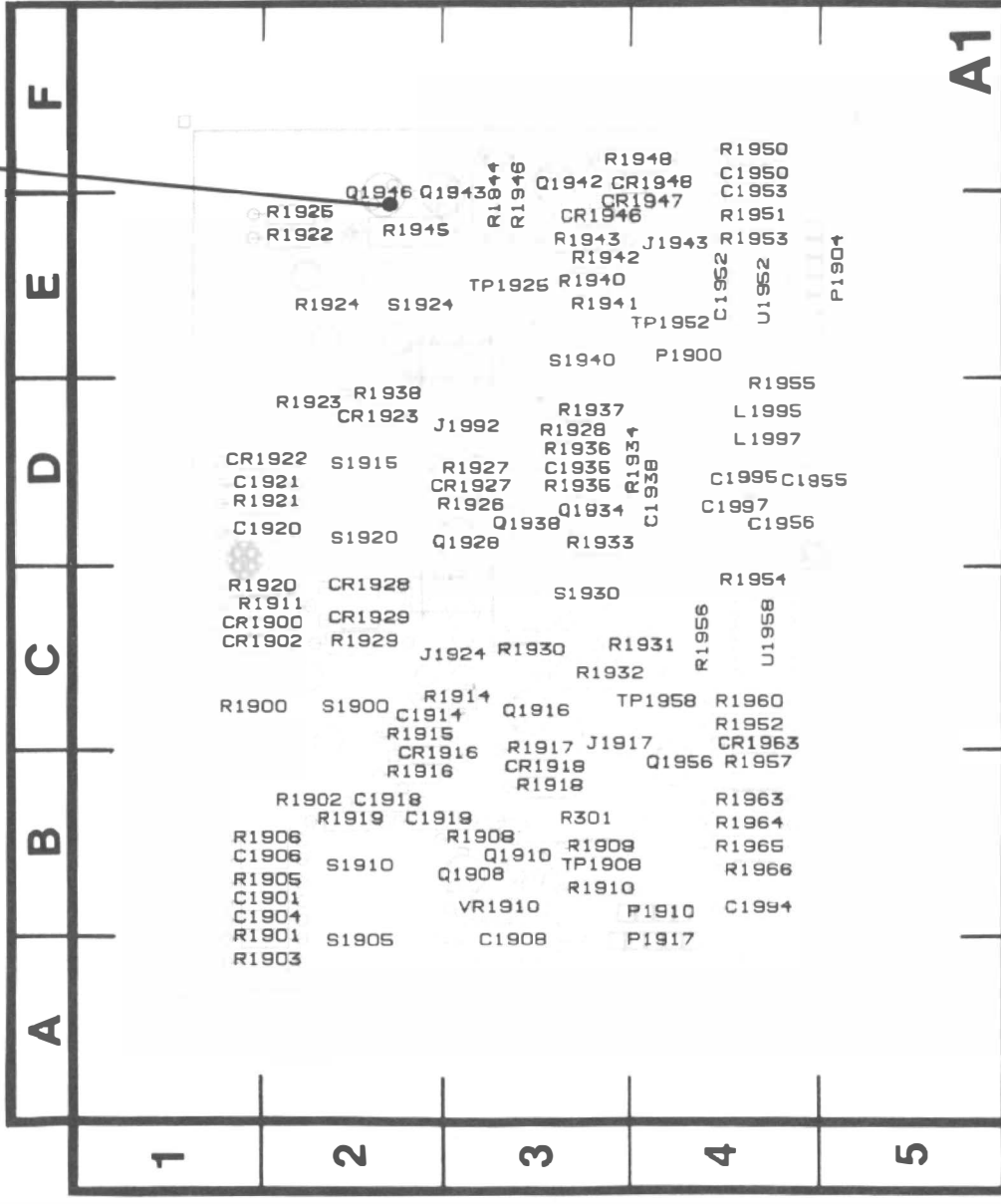
Figure 8-10. A1—Front Panel circuit board assembly.
