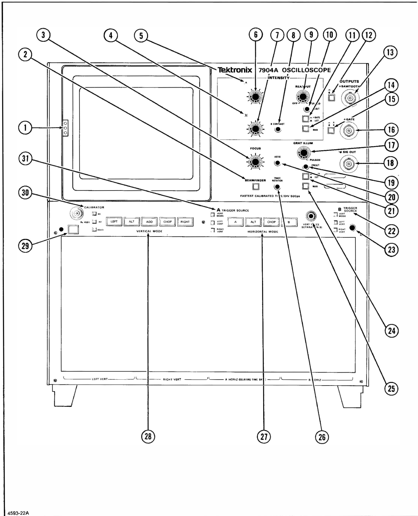
Figure 2-1. Front-panel controls, connectors and Indicators.
