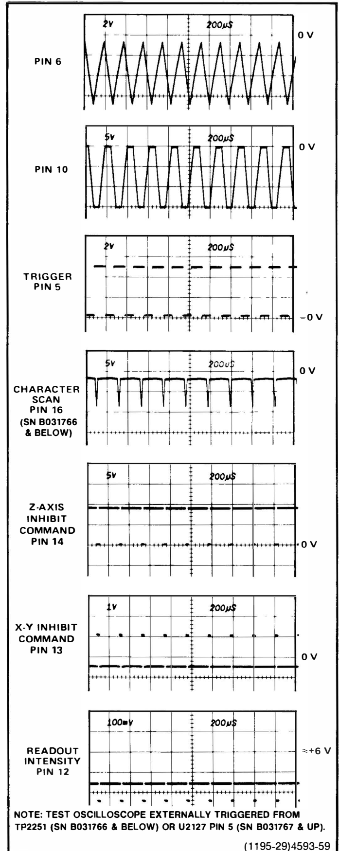
Figure 3-11. Output waveforms of the Timer stage.
