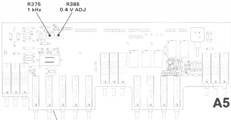
Figure 8-24. Adjustment Locations C.
