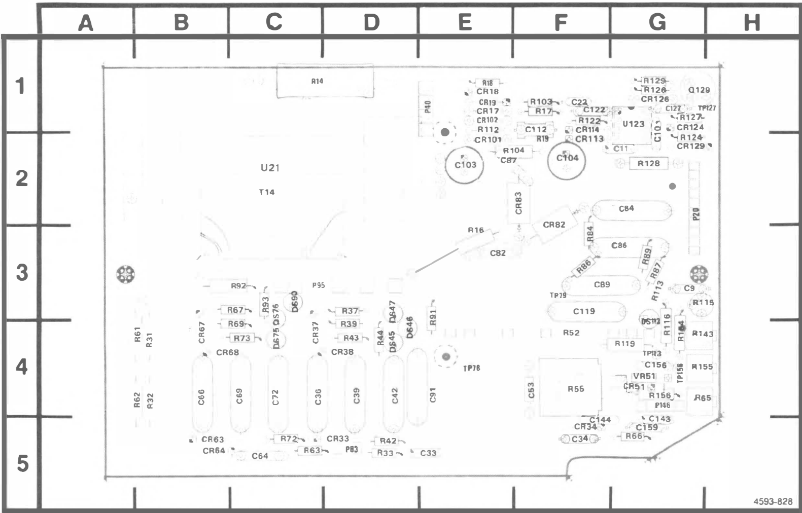
Figure 8-17A. A20—High Voltage circuit board assembly (SN B021130 & above).
