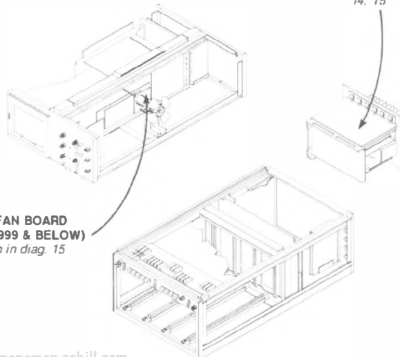
A22 LOW VOLTAGE REGULATOR BOARD Shown in diag. 14, 15
