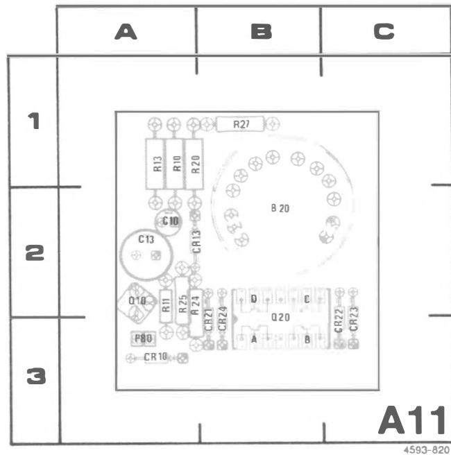
Figure 8-21. A11—Fan circuit board assembly (SN B039999 & Below).
