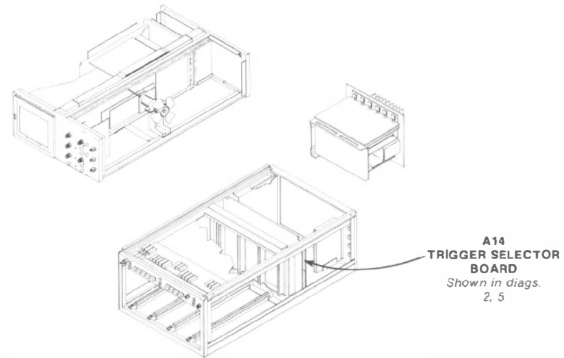
Figure 8-7. A14—Trigger Selector circuit board assembly.
