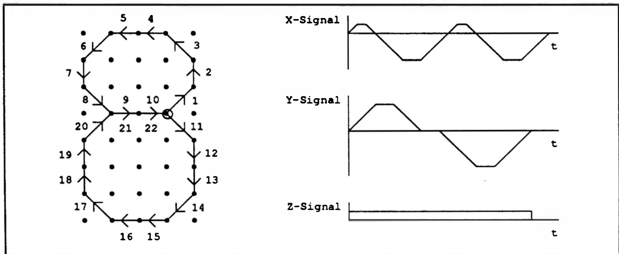
Fig. 4 Signals needed to write an "8"
