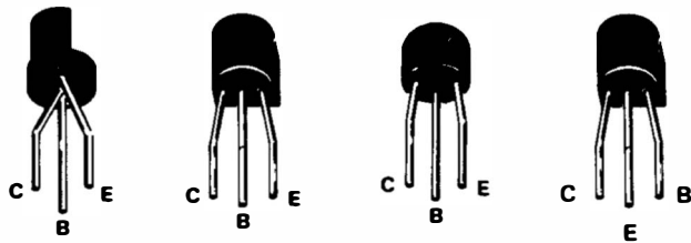
PLASTIC-CASED TRANSISTORS
