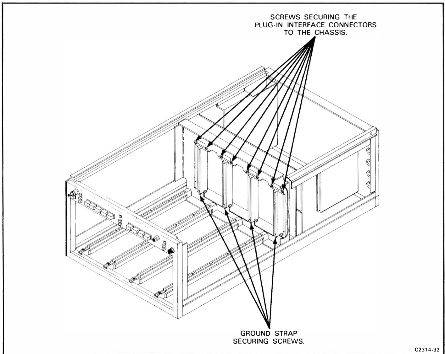
Figure 4-12. Location of securing screws for the A6-Main interface board.
