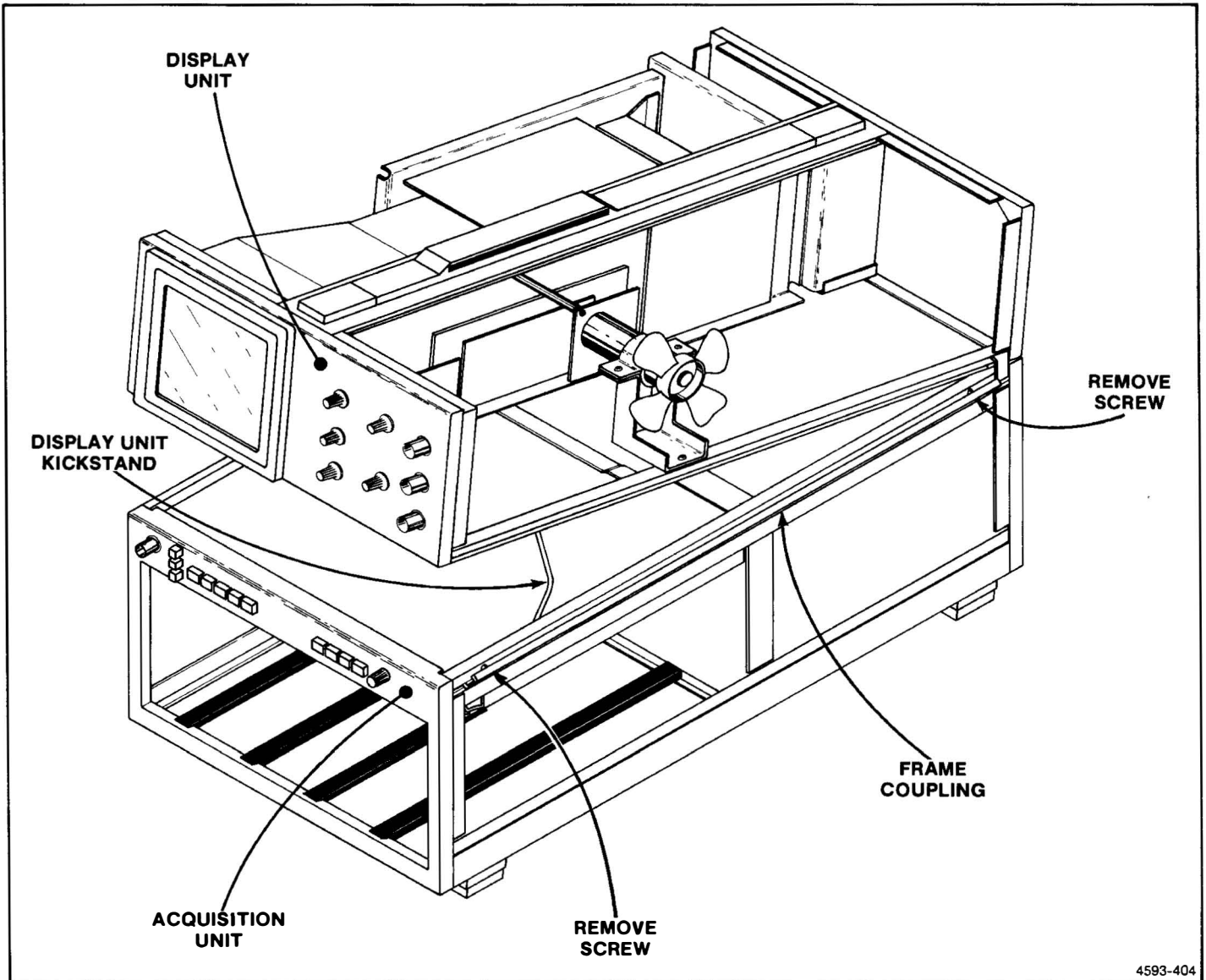
Figure 4-10. Use of Display Unit kickstand.
