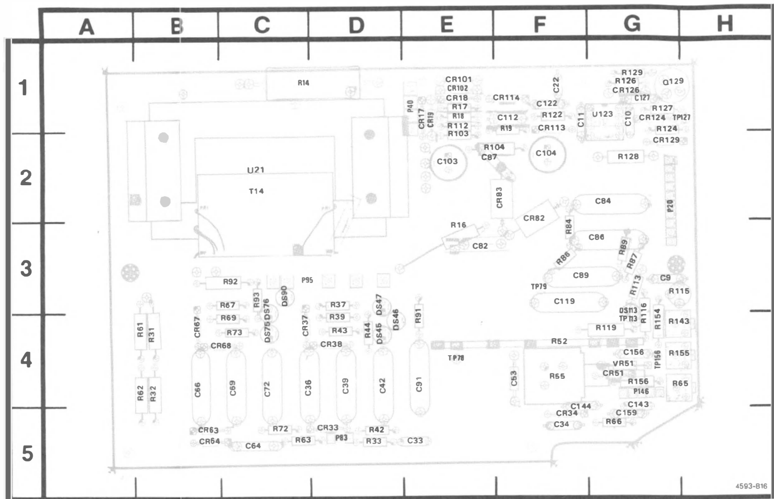
Figure 8-17B. A20—High Voltage circuit board assembly (SN B021129 & below).
