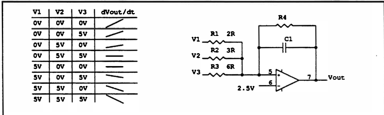
Fig. 6 a) possible codes b) Extended Integrator circuit
