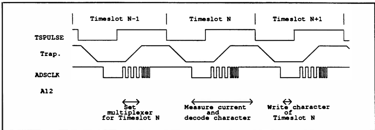
Fig. 2 Timing relations of important signals
