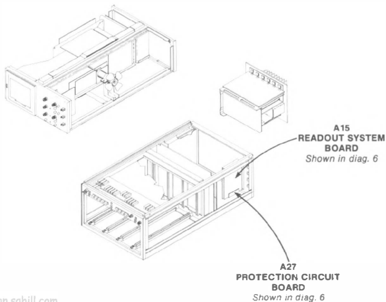
Figure 8-8B. A27—Readout Protection circuit board assembly
