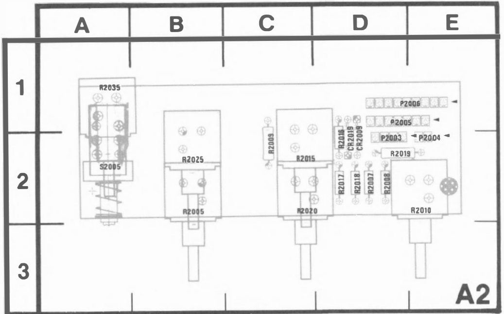
Figure 8-4. A2—Display Control circuit board assembly.
