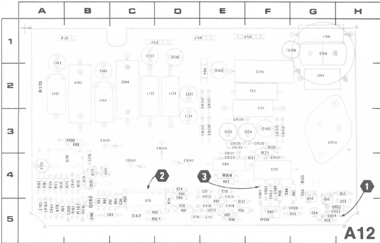
Figure 8-19. A12—Control Rectifier circuit board assembly.
