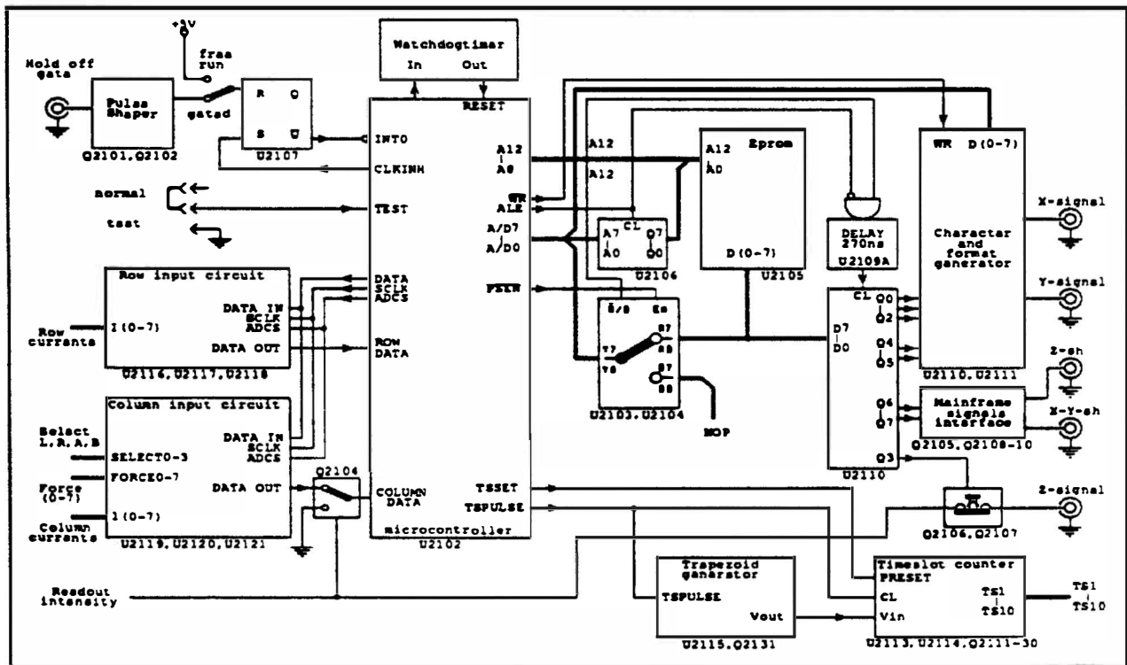
Fig. 1 Block diagram of the Readout System
