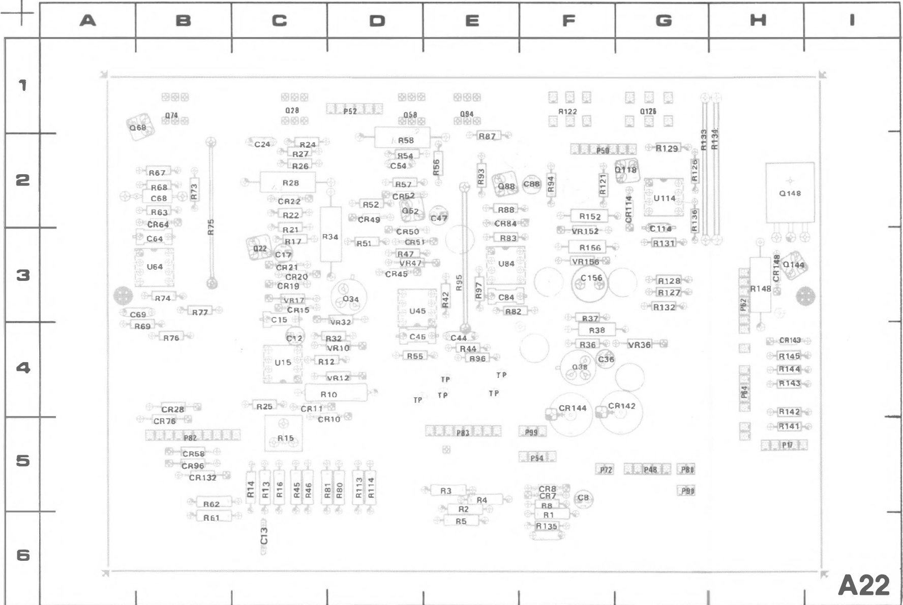
Figure 8-20. A22—Low Voltage Regulator circuit board assembly.
