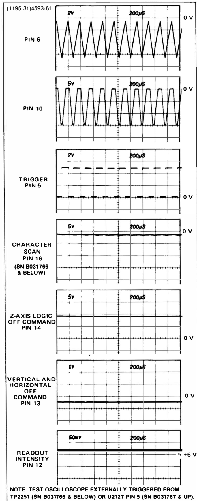
Figure 3-13. Timer stage operation when display-skip condition occurs.
