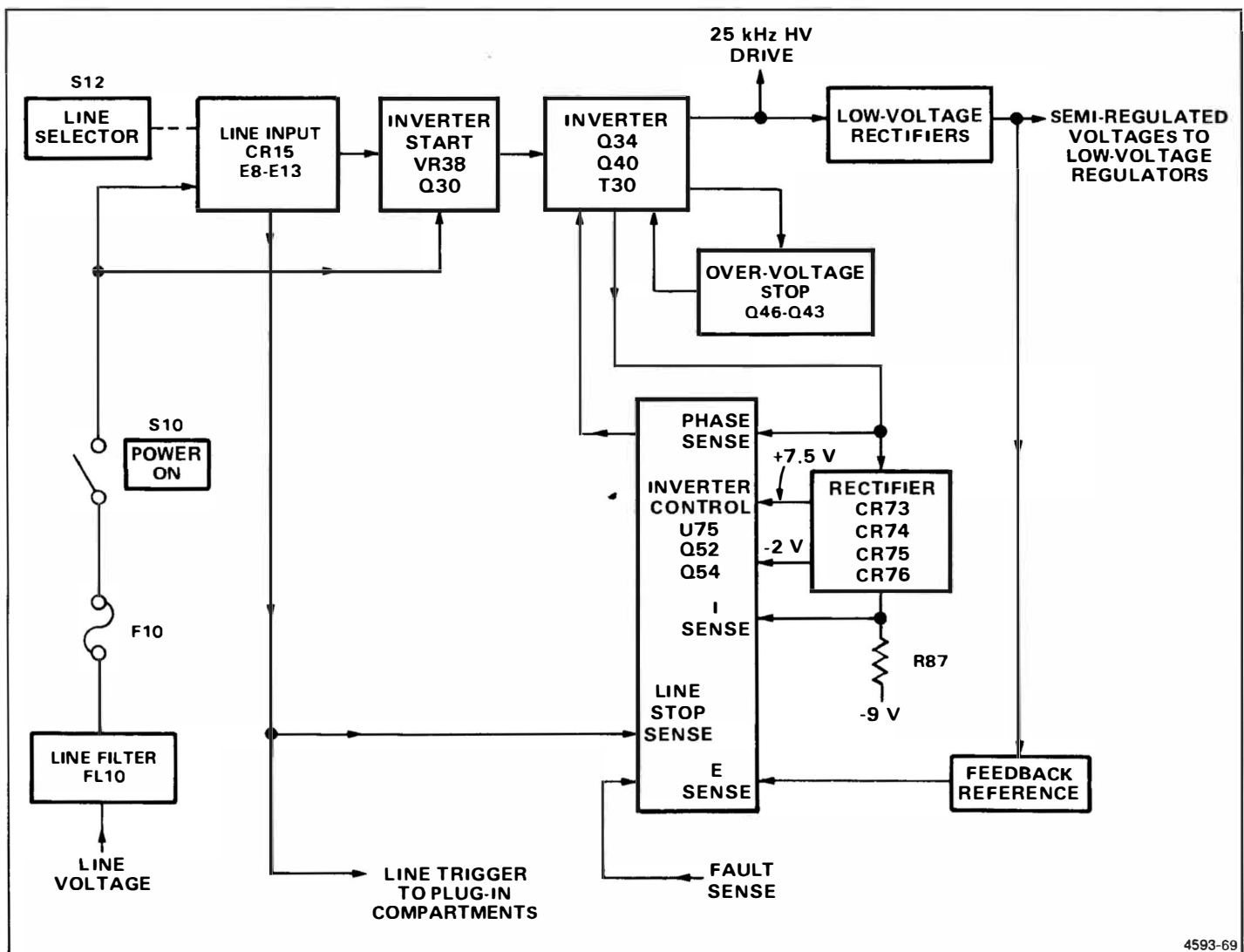
Figure 3-23. Detailed block diagram of the Converter/Rectifiers circuit.
