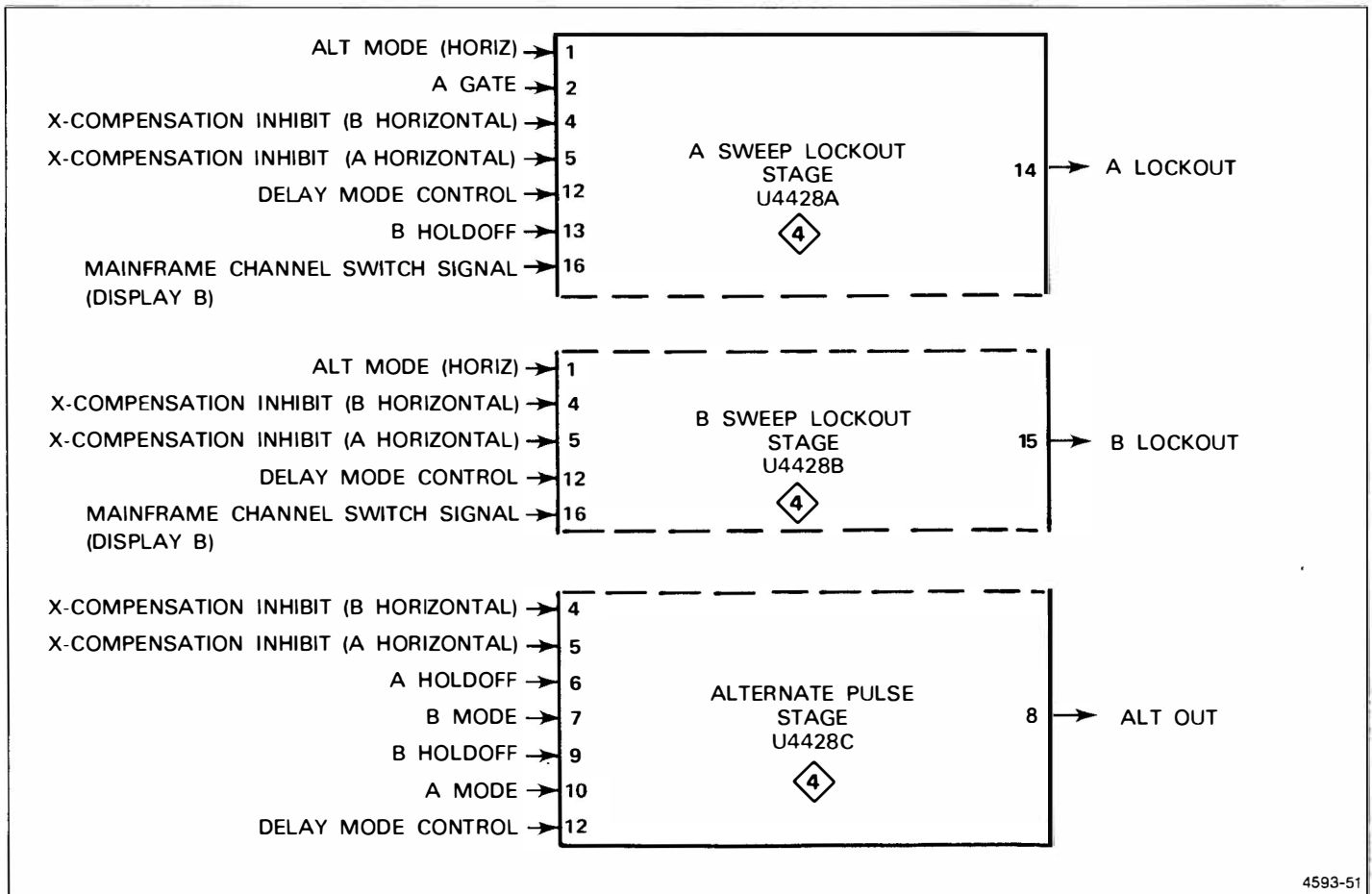
Figure 3-2. Breakdown of separate stages within Horizontal Logic IC (U4428).
