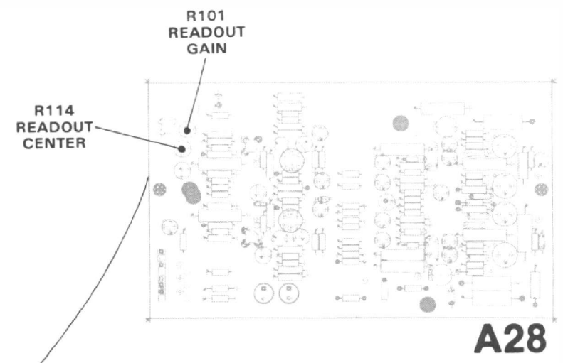
A28 HORIZONTAL AMPLIFIER BOARD Shown in diag. 11
