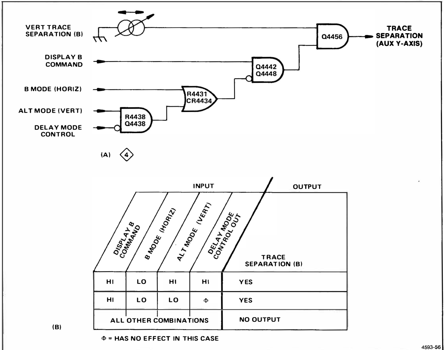
Figure 3-7. (A) Logic diagram of Trace Separation stage; (B) Table of input/output combinations.
