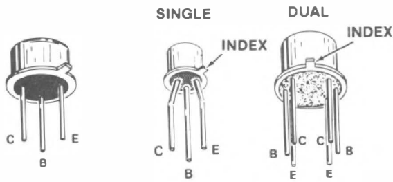
METAL-CASED TRANSISTORS
