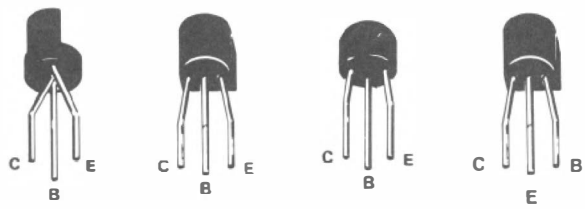
PLASTIC-CASED TRANSISTORS
