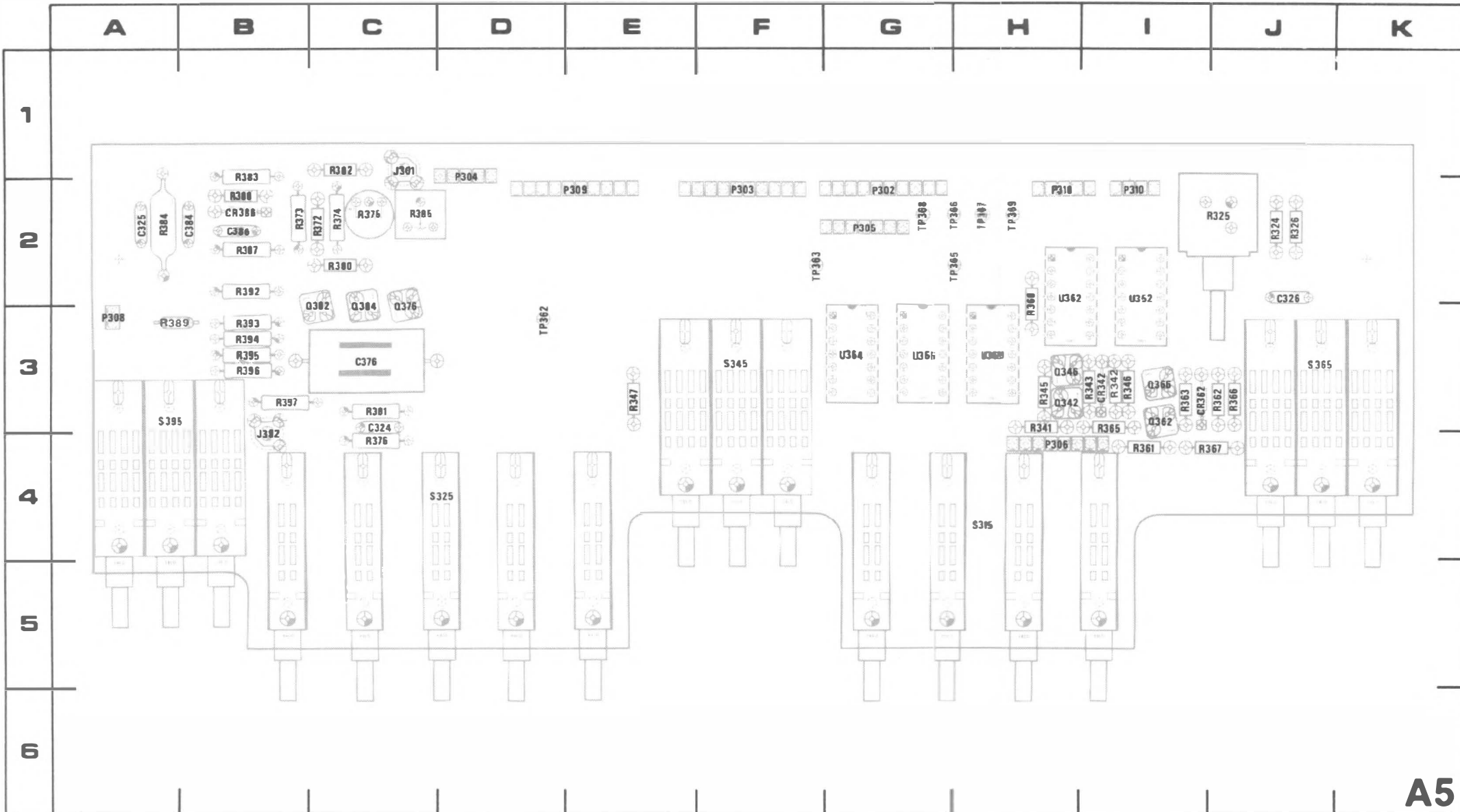
Figure 8-3. A5—Mode Switch circuit board assembly.
