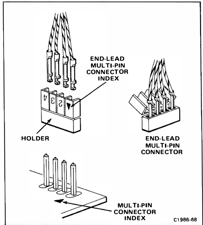
Figure 4-3. Orientation of multi-pin connectors.
