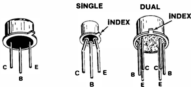
METAL-CASED TRANSISTORS
