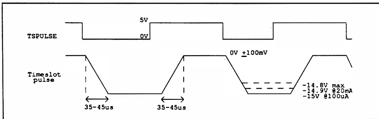
Fig. 3 The timeslot trapezoid
