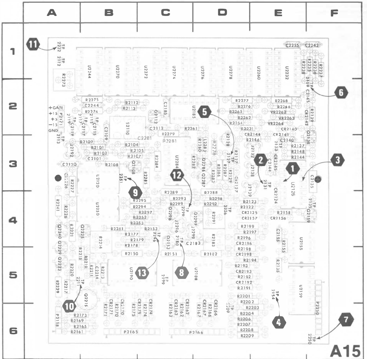
Figure 8-9. A15—Readout System circuit board assembly (SN B031766-Below)
