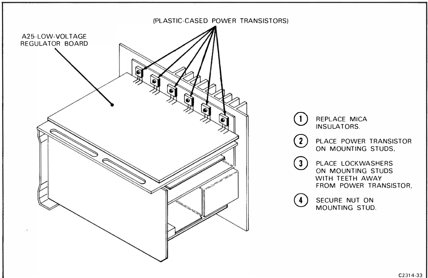
Figure 4-13. Correct placement of power transistor and mounting hardware on rear heatsink.
