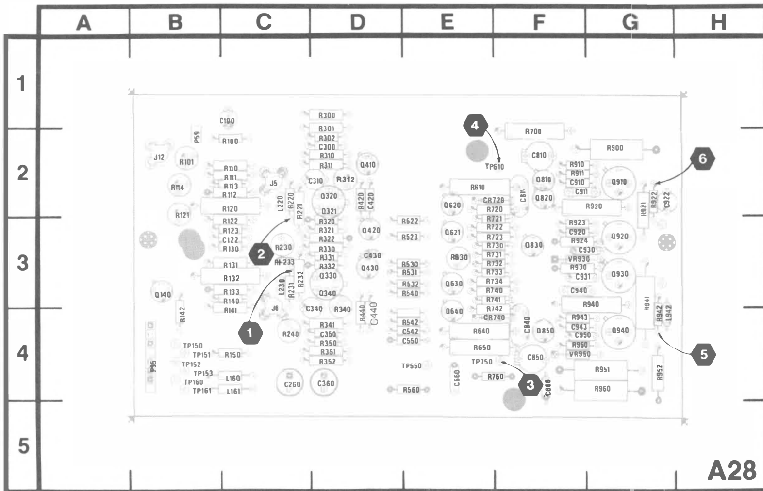
Figure 8-15. A28—Horizontal Amplifier circuit board assembly.
