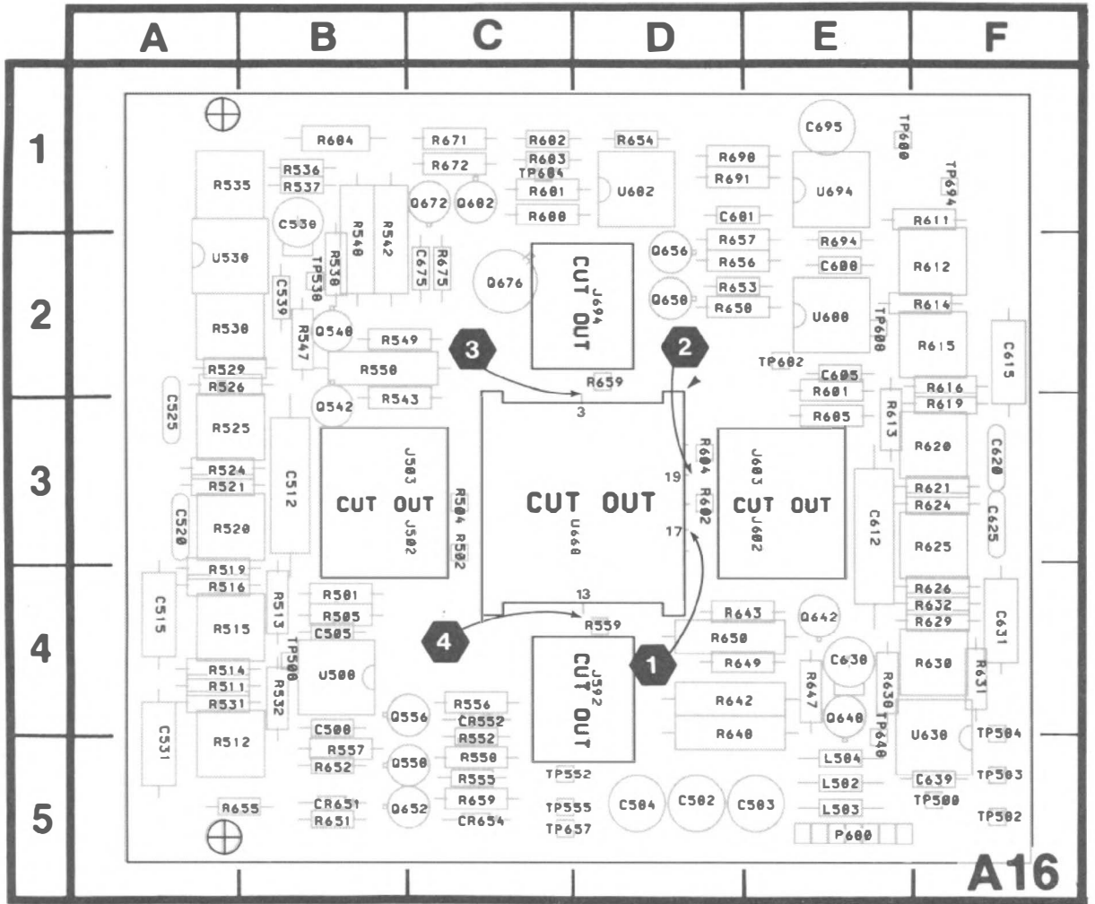
Figure 8-11. A16—Vertical Channel Switch circuit board assembly.
